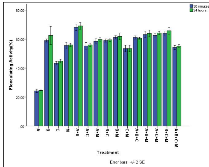
Fig. 3. Flocculating activities of abattoir waste water sample with different treatment combinations
