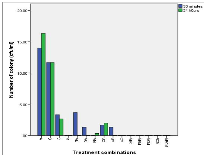
Fig. 9. Effect of various treatment combinations on the number of bacteria growth on NA for abattoir waste water sample Key A- Alum B- Bioflocculant C-Chlorine M-Moringa
