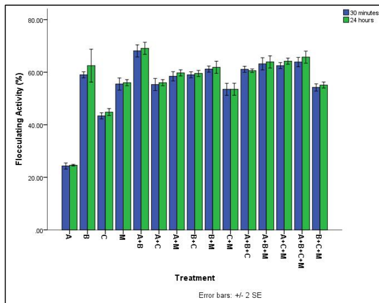
Fig. 1. Flocculating activities of well water samples treated with different Combinations KEY A- Alum B- Bioflocculant C-Chlorine M-Moringa
