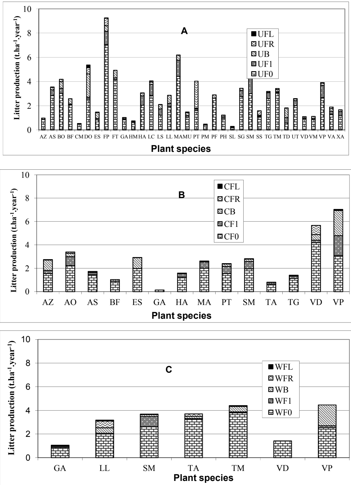
Fig. 1. Litter production by category ( t \cdot ha^{-1} \cdot yr^{-1} ) at Dang (A), Biskewal (B) and Wakwa (C). Leaf litter of year n (F0), previous years (F1), wood litter (B), fruits and seed litter (FR), and Flower litter (FL). Dang (U), Biskewal (C), and Wakwa (W)
