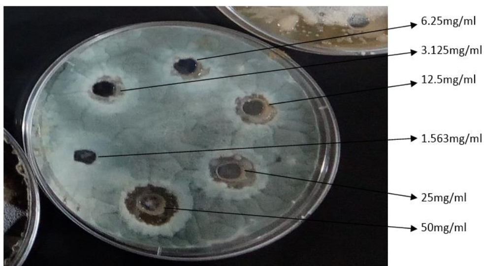
Fig. 2. Inhibition Zone Diameters of the Different Concentrations of Shampoo against Microsporium ferrugineum
