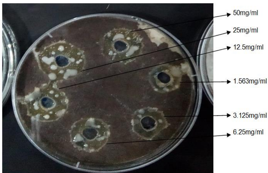
Fig. 1. Inhibition Zone Diameters of the Different Concentrations of Miconazole against Trichophyton mentagrophytes
