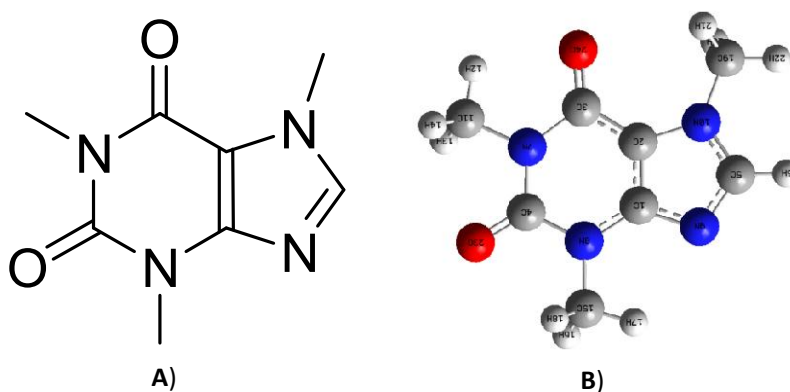
Fig. 7. A) Chemical structure used to model Caffeine, B) optimized structure of caffeine at B3LYP/6-31G(d) level
