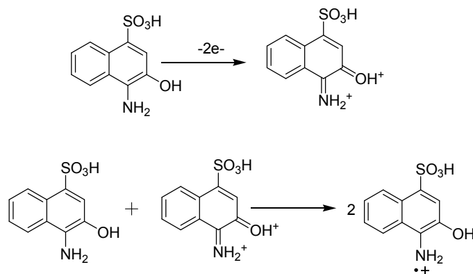
Scheme 3. Proposed mechanism for formation of AHNSACR via disproportionation redox reaction
