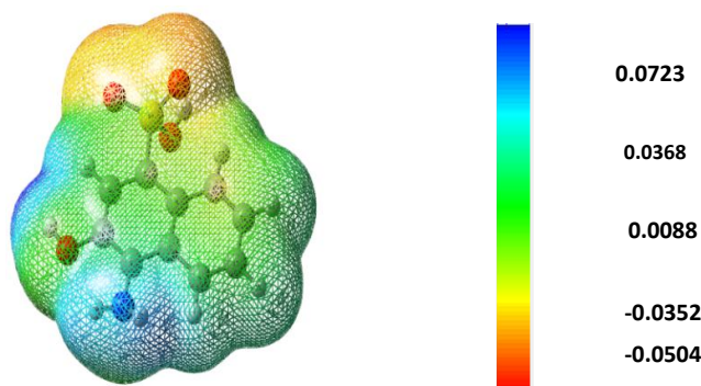
Fig. 5. Molecular Electrostatic Potential (MEP) surface of AHNSA calculated at the B3LYP/6-31G(d) method
