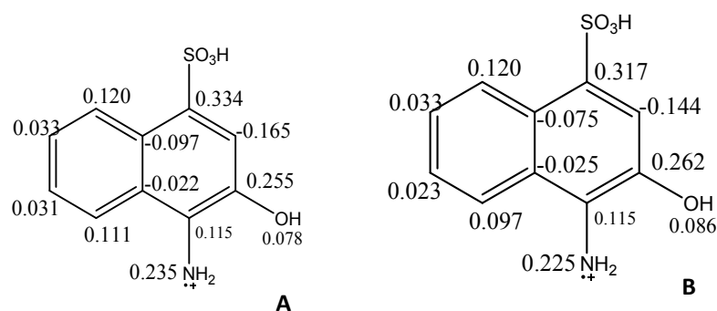
Scheme 5. Total Spin densities distribution of AHNSACR calculated at: A) B3LYP/ 6-31G(d) and B) B3LYP/ 6-31G(d) levels
