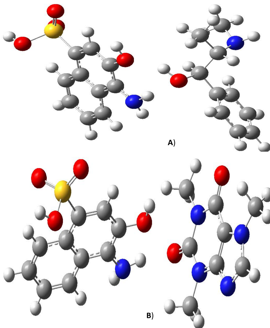
Fig. 8. Optimized binding structures of A) AHNSA – ephedrine, and B) AHNSA - caffeine complexes calculated at B3LYP/6-31G(d)
