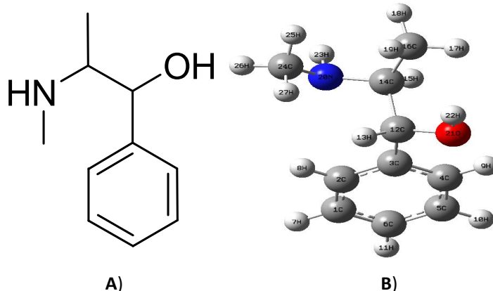
Fig. 6. A) Chemical structure used to model Ephedrine, B) optimized structure of ephedrine at B3LYP/6-31G(d) level
