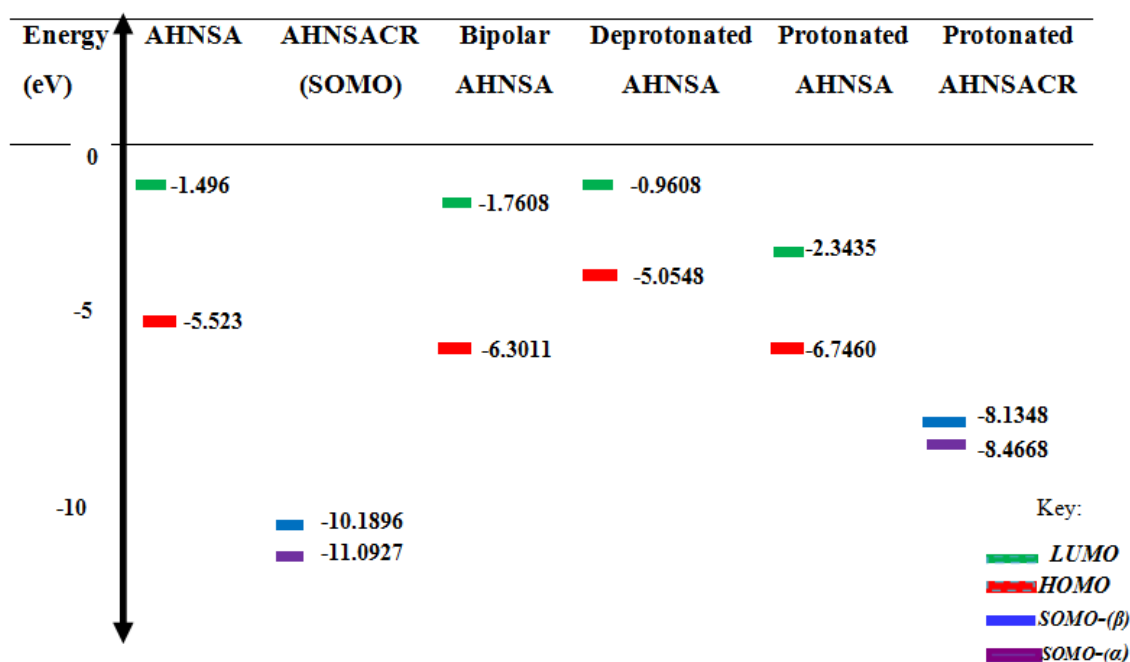
Fig. 4. Energy diagram and illustrations of AHNSA, AHNSACR, bipolar AHNSA, deprotonated AHNSA, protonated AHNSA, and protonated AHNSACR molecular orbitals, obtained using DFT/(B3LYP/6-31G(d)) methodology within a 0.02 isosurface cutoff approximation
