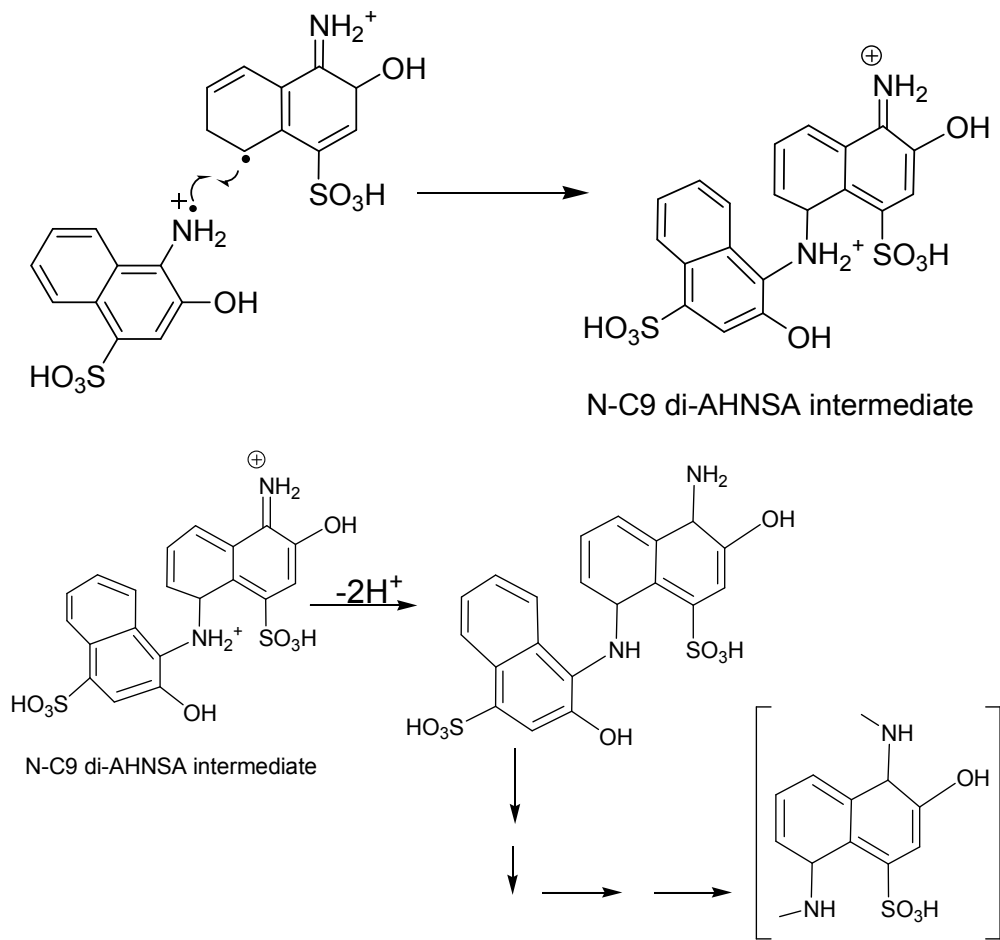
Scheme 7. Proposed polymerization mechanism for AHNSA through N-C9 coupling reactions
