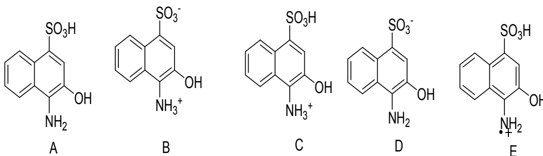
Scheme 2. Structures used to model A) AHNSA, B) zwitterionic AHNSA, C) protonated AHNSA, D) deprotonated AHNSA, and E) AHNSA radical cation
