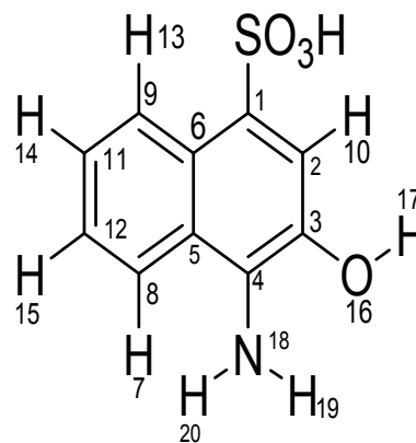
Scheme 1. Molecular structure and numbering scheme of AHNSA
