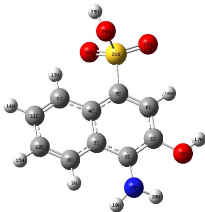
Fig. 1. Optimized structure of AHNSA
