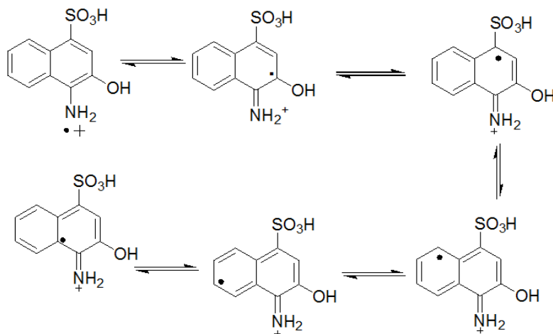
Scheme 4. Pictorial representation of spin density delocalization of AHNSACR
