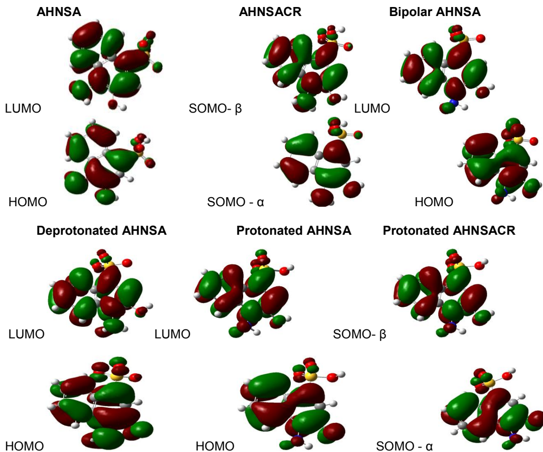
Fig. 3. Schematic representation of different forms AHNSA orbitals involved in the coupling calculated at B3LYP/6-31G(d) level of theory, within a 0.02 isosurface cutoff approximation
