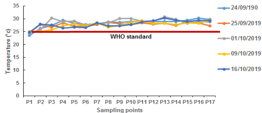
Fig. 4. Temporal variation of the temperature according to the sampling points of the North zone
