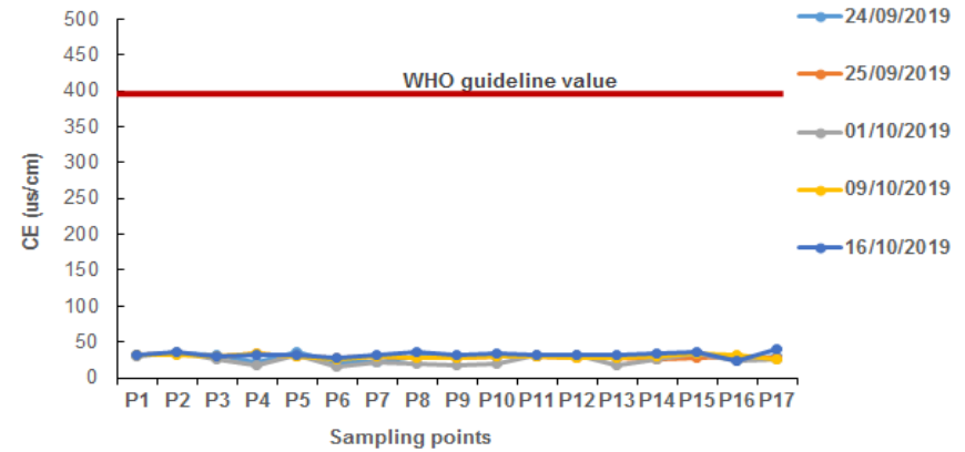
Fig. 12. Temporal variation of the conductivity according to the sampling points of the North
