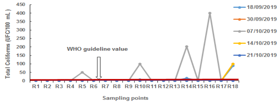
Fig. 15. Temporal variation of total coliforms according to sampling points in the South zone
