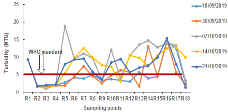
Fig. 7. Temporal variation of turbidity according to points sampling from the South zone
