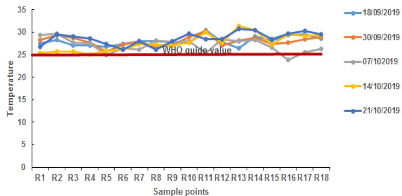
Fig. 3. Temporal variation of the temperature according to the sampling points of the South zone
