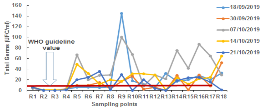
Fig. 13. Temporal variation of total germs according to sampling points in the South zone
