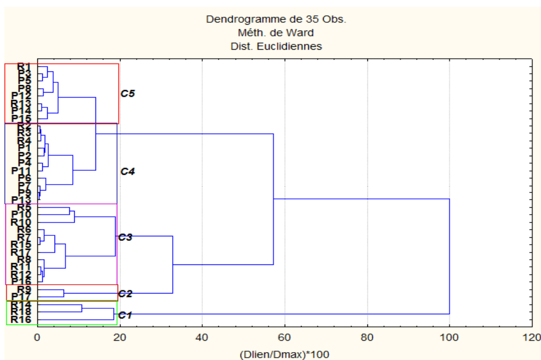
Fig. 19. Classification dendrogramme of tap water sampling points
