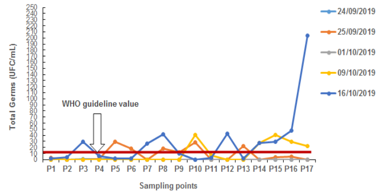
Fig. 14. Variation of total germs according to points collection from the North zone
