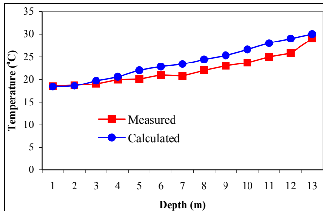
Fig. 10. Comparison of calculations and experiments for saturated soil with groundwater flow (SSG)
