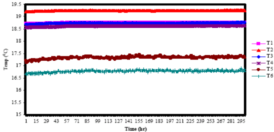
Fig. 17. Variation of temperatures for heat exchanger for two weeks
