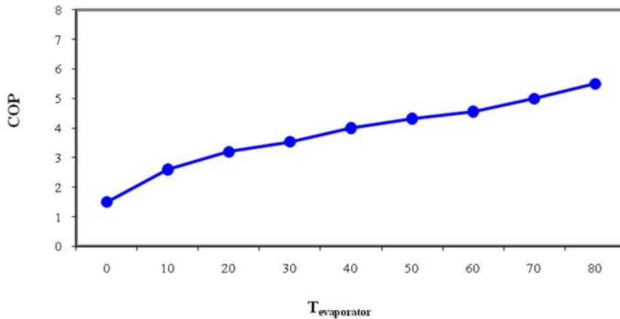
Fig. 6. Heat pump performance vs evaporation temperature
