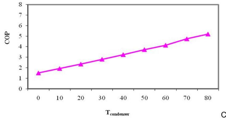
Fig. 7. Heat pump performance vs condensation temperature
