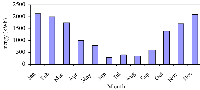
Fig. 22. Monthly heating energy demands
