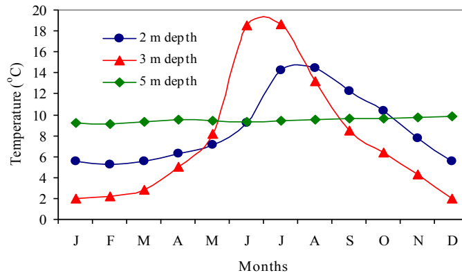
Fig. 8. Seasonal temperature variations
