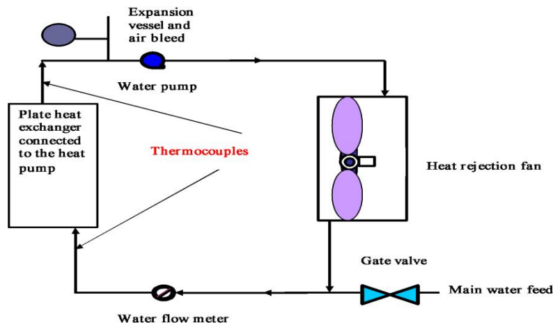
Fig. 1. Sketch of installing heat pump
