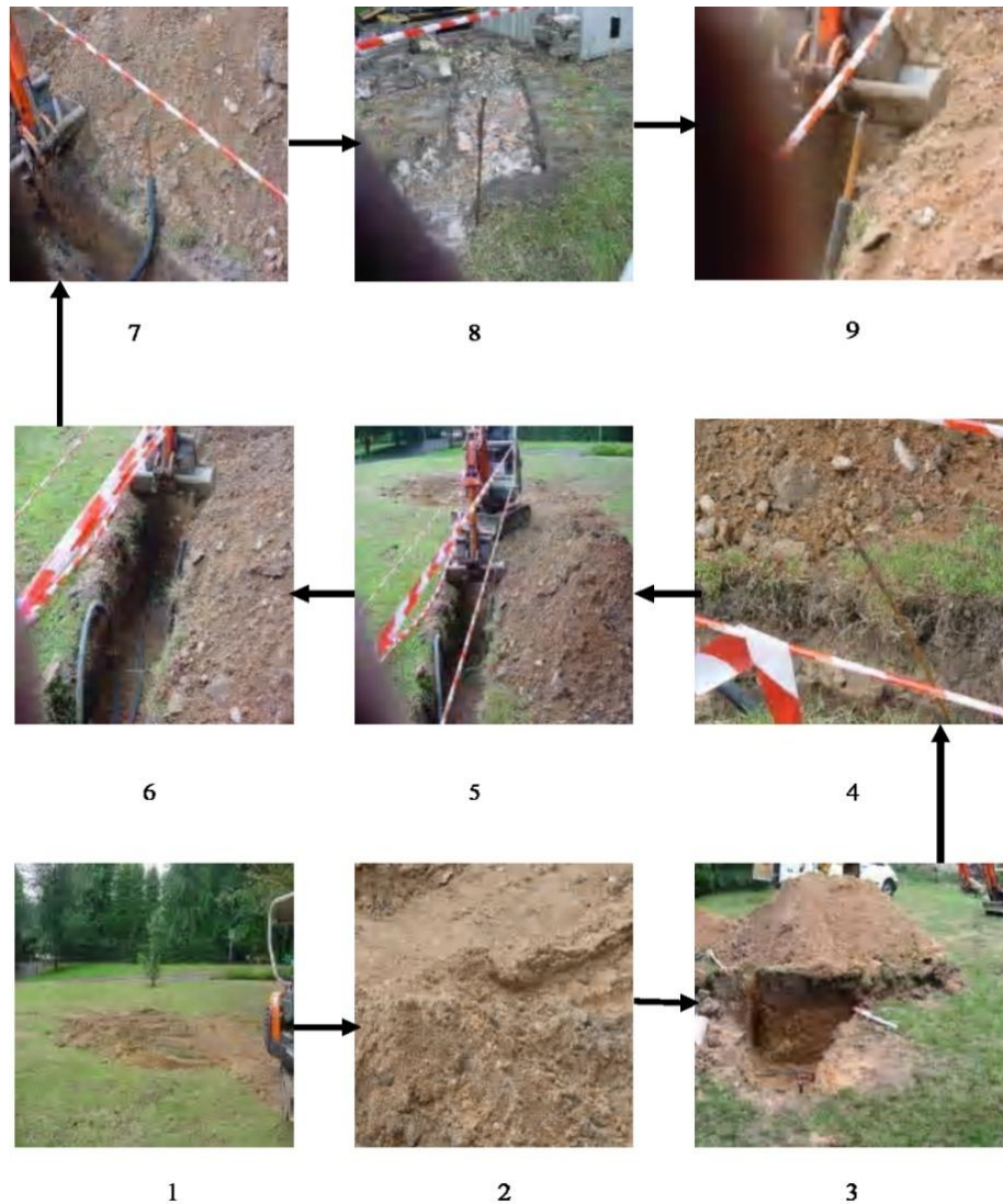
Fig. 3. Showing the drilling (1-2) digging of the pit (3), connection of the manifolds (4), grouting, preparation of the coils (5-6) and the source loop, which consists of two earth loops: one for vapour and one for liquid (7-9)
