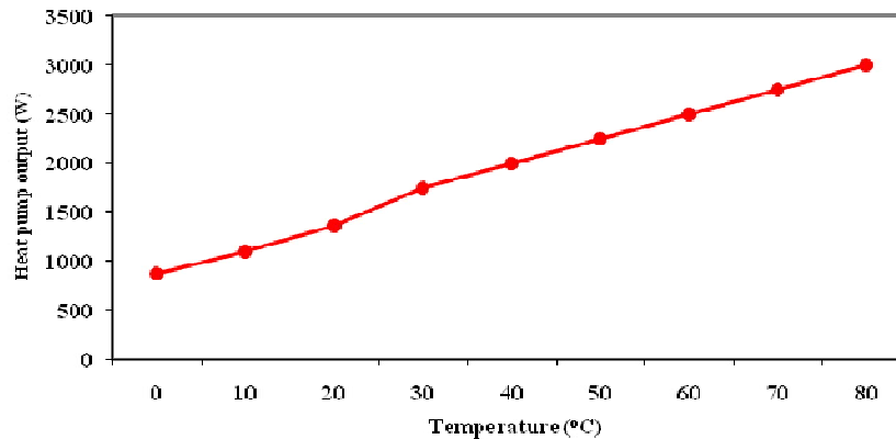
Fig. 20. Variation of heat pump output with temperature
