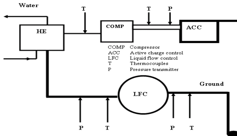
Fig. 2. Shows the connections of ground loops to heat pump and heat exchanger (HE)
